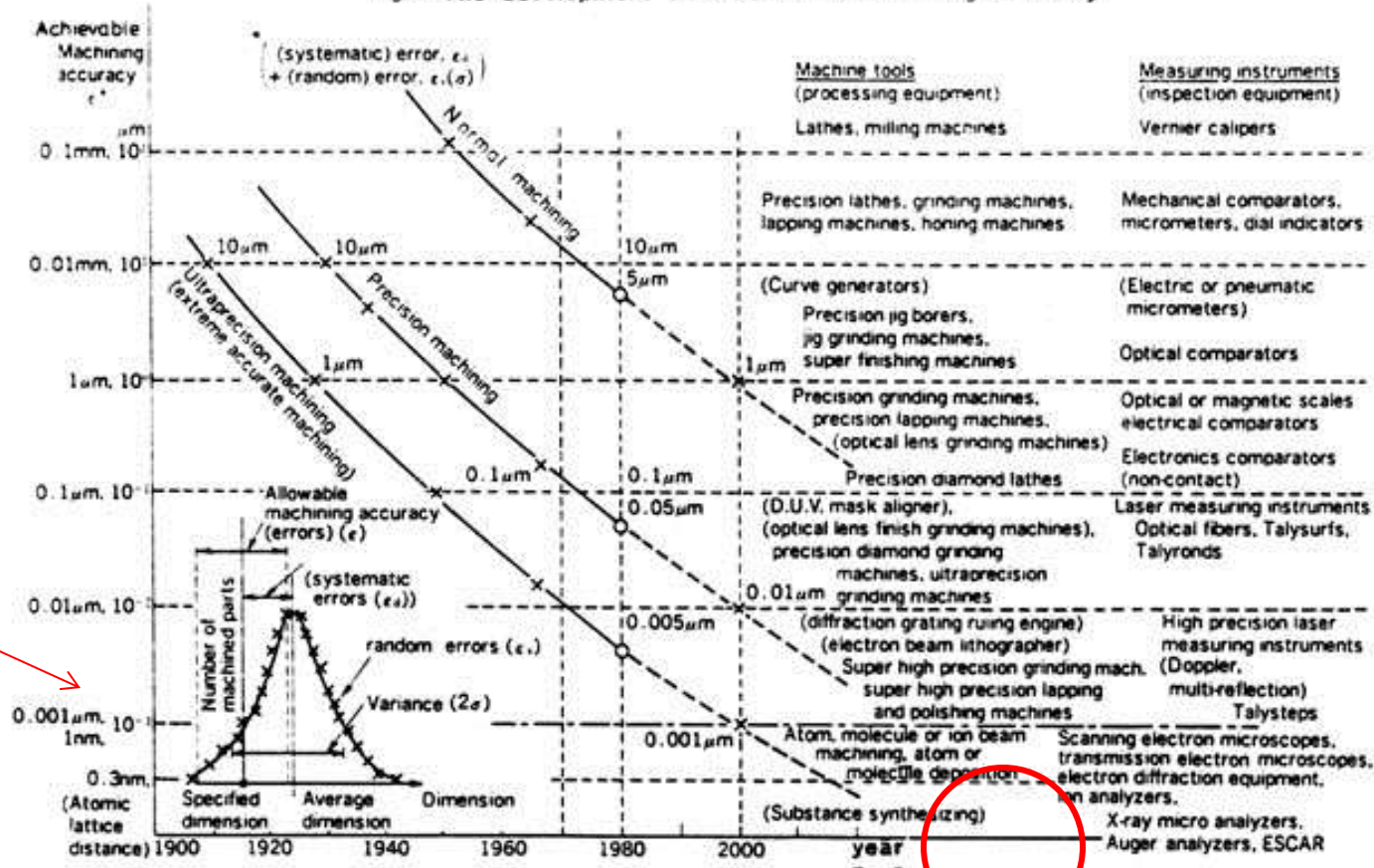
Fig.1 The development of achievable machining accuracy
