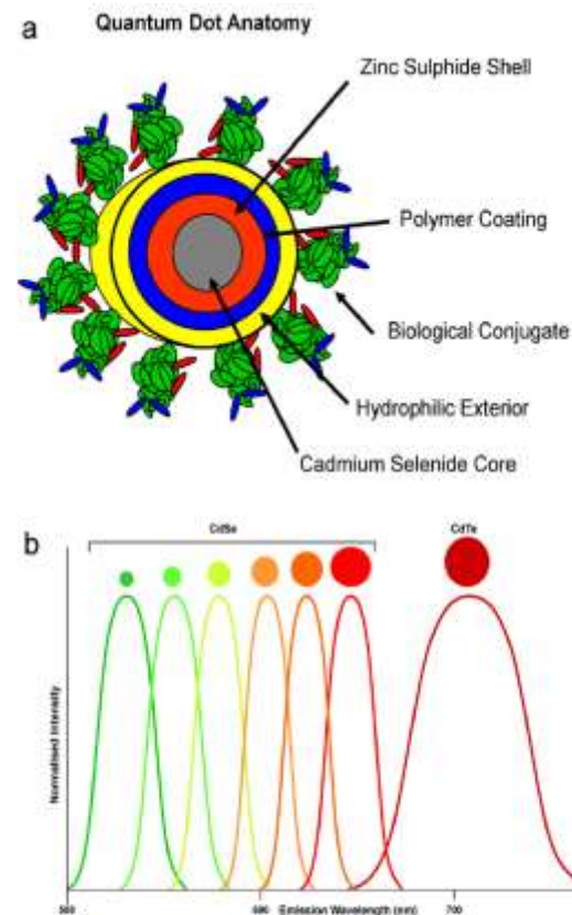
Figure 1. (a) Schematic representation of a QD Quantum dots are composed of a Cadmium Selenide (CdSe) core, around which a Zinc Sulphide (ZnS) shell is added to increase quantum yield. Addition of polymer and hydrophilic coverings is required for stability and the outside of the assembly is coated with biomolecules such as streptavidin or amine to enable attachment to other molecules (reproduced with permission from Tholouli et al , J Pathol 2008, 216, 275-285).
